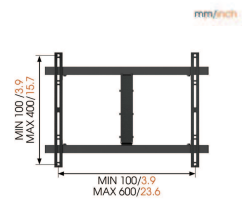
VESA mounting holes mm/inch
